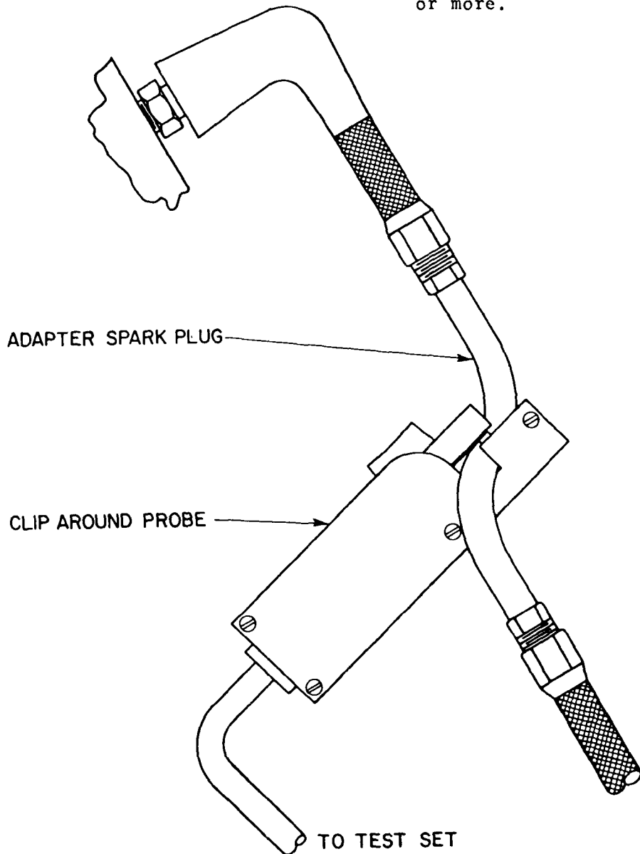
FIG 2-2. TACHOMETER CONNECTION
